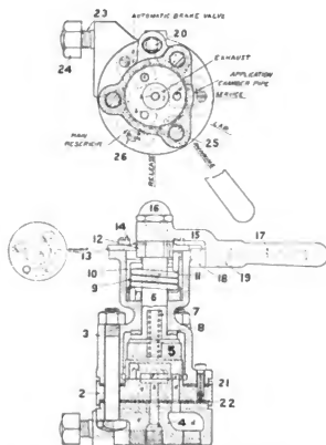
Figs. 2474-2476. Westinghouse S F Independent Engineer's Brake Valve.
